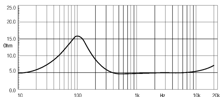
FREE AIR IMPEDANCE MAGNITUDE CURVE - AIC ON
