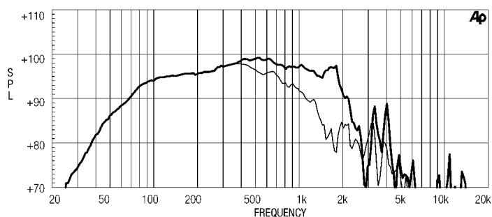
FREQUENCY RESPONSE CURVE OF 15LW1401 MADE ON 125 LIT. ENCLOSURE TUNED 50HZ IN FREE FIELD (4PI) ENVIRONMENT. ENCLOSURE CLOSES THE REAR OF THE DRIVER. THE THIN LINE REPRESENTS 45 DEG. OFF AXIS FREQUENCY RESPONSE
