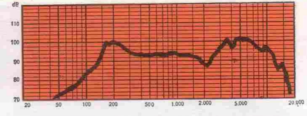
CIS 17 D 166 mm - 6 1/2" 3 W
