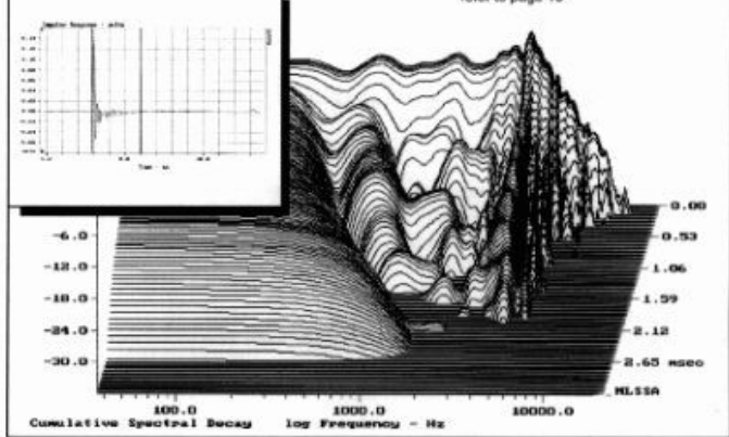
IMPULSE RESPONSE WATERFALL refer to page 16
