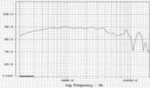
Frequenzgang/Amplitude response
