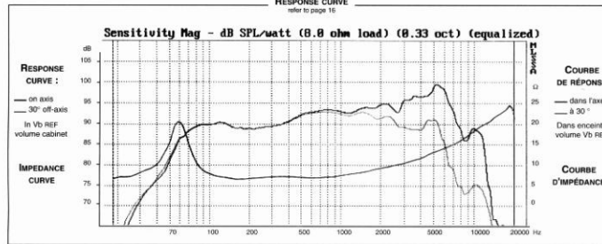
RESPONSE CURVE refer to page 16
