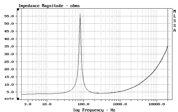
Impedance
