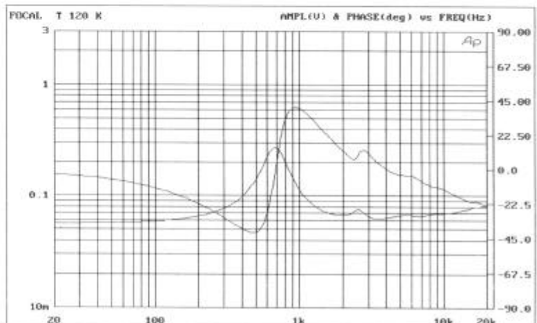
Impedance magnitude and phase versus frequency
